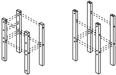
(A) Upper Post (Shorter) x 4 (B) Lower Post (Longer) x 4
